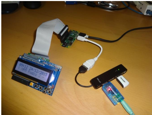
Figure 14 The Radio running on a Pi Zero
