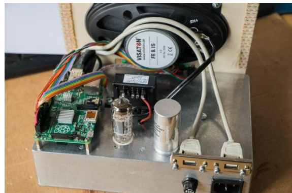
Figure 21 The RPi valve radio chassis view
