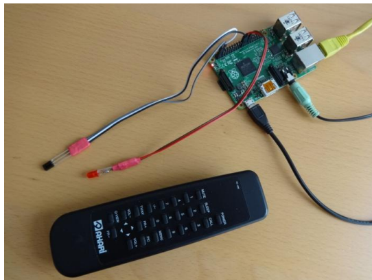
Figure 83 IR Sensor and Remote control
