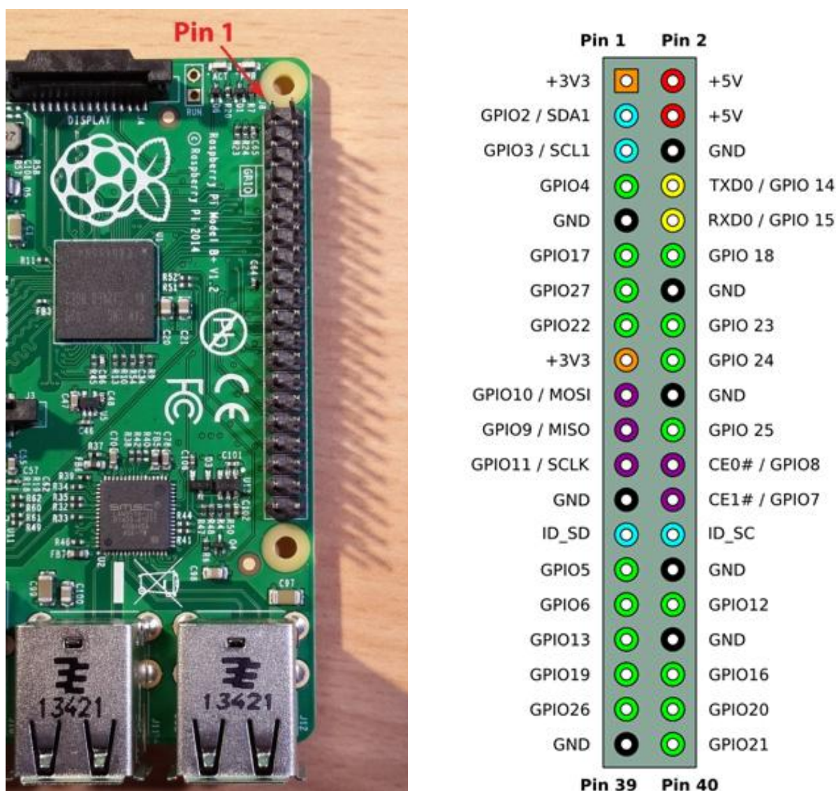
Figure 103 GPIO Pin Numbers
