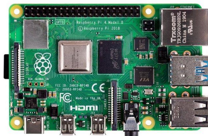
Figure 30 Raspberry Pi Model 4B Computer
