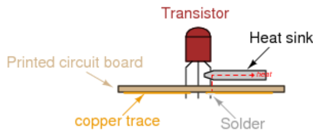
Figure 118 Soldering precautions
